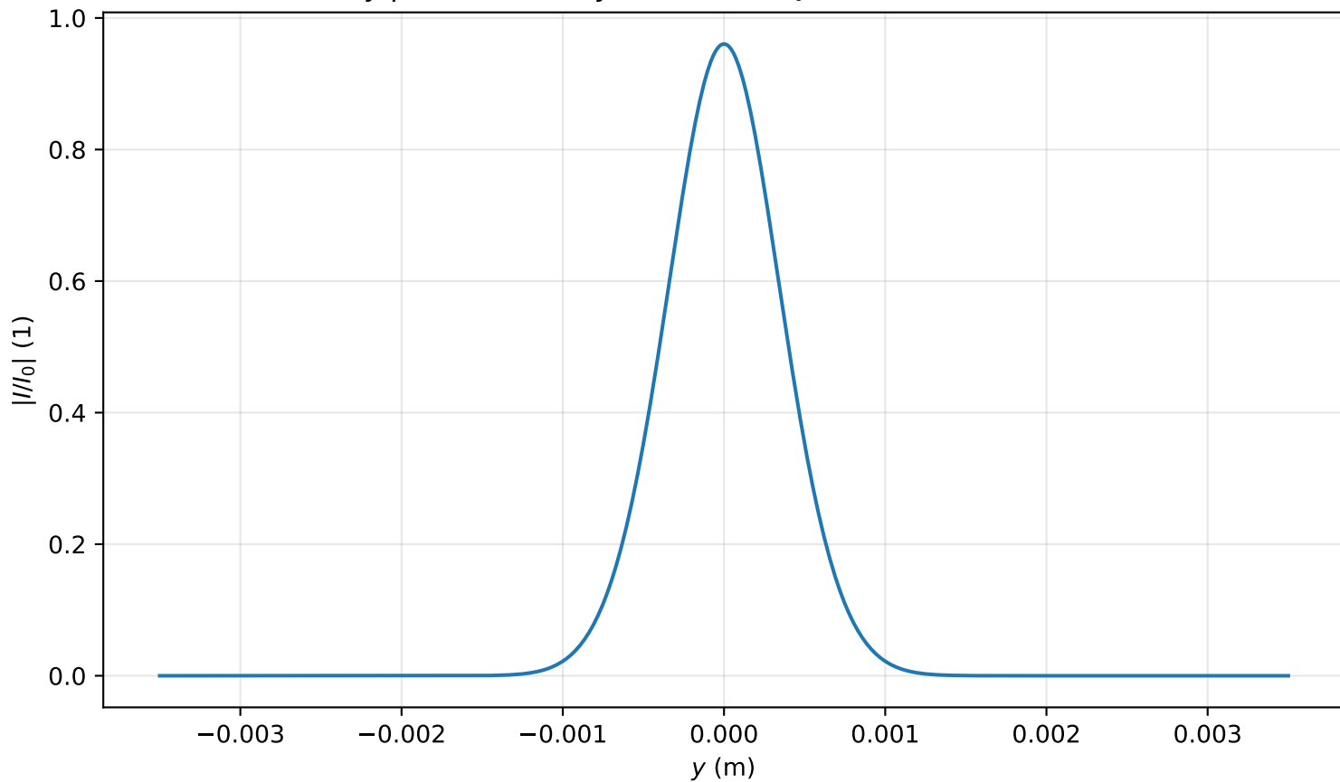
Intensity profile I(x=0, y, z=0.637)/I_0 , P_{in}=0.2P_{cr} , artificial time
